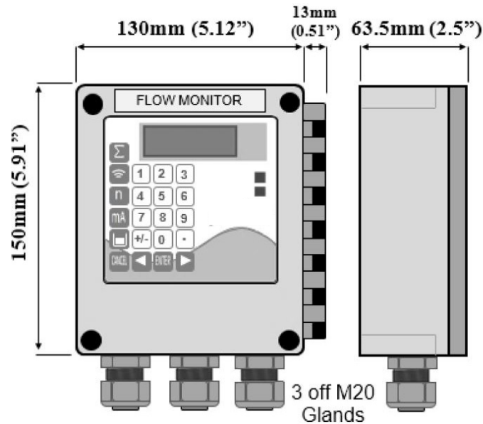
Flow Monitor Front and Side Drawing
