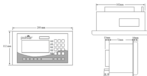
Ultra 5 Fascia Mount Drawings Front, Top and Side
