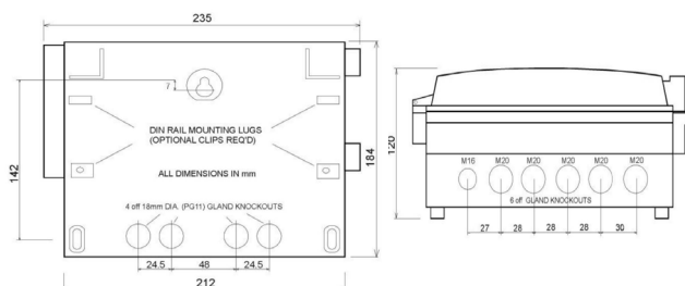
Ultra 5 Wall Mount and Gland Knockouts
